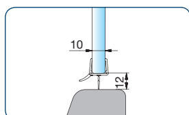
art. no. 8864KU0-12-2500 for 10 and 12 mm glass
