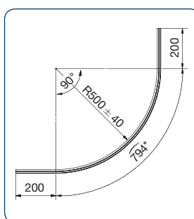
art. no. 8867KU0-8-R500 curved for tube radius R500 - 550 for 6 and 8 mm glass winding off = 1194 mm
