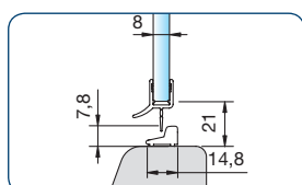
art. no. 8590E6EV5-2010 Splash guard in square design, length 2010 mm with sealing profile 8864KU0-8-2010
