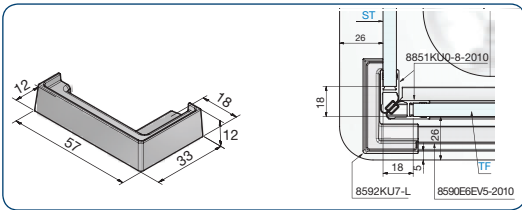
art. no. 8592KU7-L 90° cover cap left
