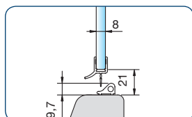
art. no. 8864KU0-8-2010 for 6 and 8 mm glass in combination with splash guard (art. no. 8535E6EV5)
