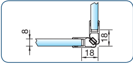
art. no. 8851KU7-8-2010 sealing profile for glass-glass 90° for 6 und 8 mm glass for an inward opening shower hinge
