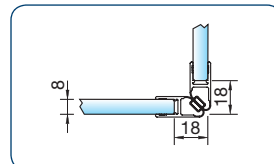
sealing profiles for glass-glass 90°
