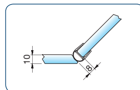
sealing profiles for glass-glass 135°
