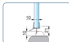
art. no. 8864KU0-12-2500 for 10 and 12 mm glass in combina- tion with acrylic semi-circular rod (art. no. 8539KU5, radius = 10 mm)
