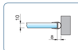
sealing profiles for door/wall 90° (hinge side)
