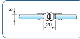
art. no. 8850KU7-8-2010 sealing profile for glass-glass 180° for 6 and 8 mm glass for an inward and outward opening shower hinge
