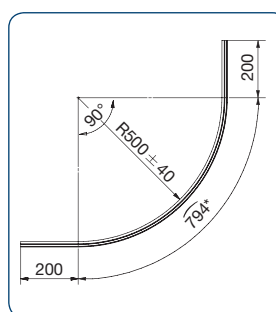
art. no. 8881E6/EV5-R500 art. no. 8882E6/EV5-R500 art. no. 8881E0/14-R500 art. no. 8882E0/14-R500
