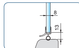
art. no. 8863KU0-8-2010 for 6 and 8 mm glass
