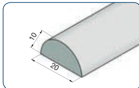
art. no. 8539KU5 splash guard with a length of 2000 mm
