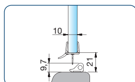
art. no. 8864KU0-12-2500 for 10 and 12 mm glass in combination with splash guard (art. no. 8535E6EV5)
