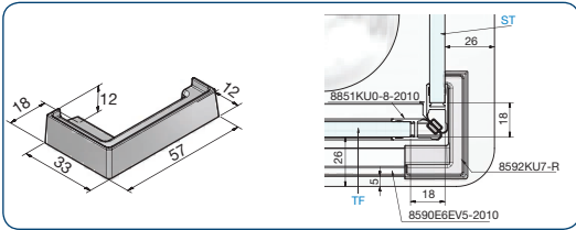
art. no. 8592KU7-R 90° cover cap right
