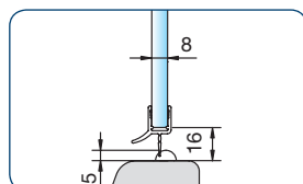
art. no. 8864KU0-8-2010 for 6 and 8 mm glass in combina- tion with acrylic semi-circular rod (art. no. 8538KU5, radius = 5 mm)
