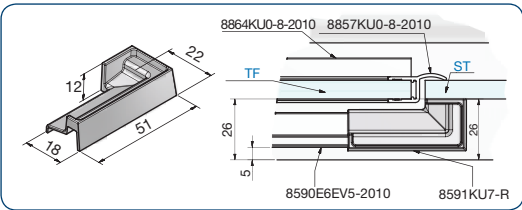
art. no. 8591KU7-R cover cap right
