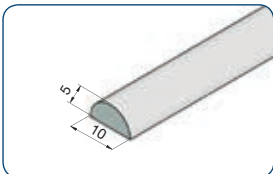
art. no. 8538KU5 splash guard with a length of 2000 mm
