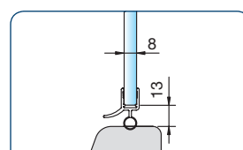
art. no. 8867KU0-8-R500 curved for tube radius R500 - 550 for 6 and 8 mm glass winding off = 1194 mm
