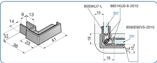
art. no. 8593KU7-L 90° connection side panel splash guard left
