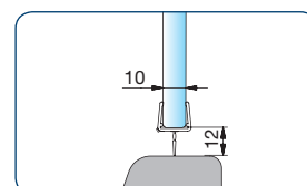
art. no. 8876KU0-12-2500 for 10 and 12 mm glass
