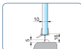
art. no. 8864KU0-12-2500 for 10 and 12 mm glass in combina- tion with acrylic semi-circular rod (art. no. 8538KU5, radius = 5 mm)
