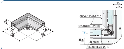
art. no. 8594KU7 90° corner connector
