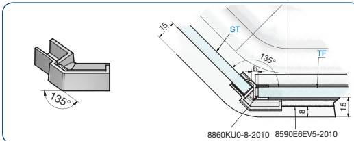
art. no. 8597KU7-R pentagonal connector right – door hinge left
