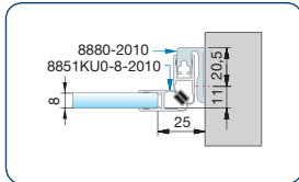
carrier profile for door stop
