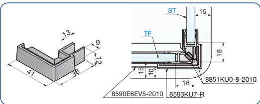
art. no. 8593KU7-R 90° connection side panel splash guard right
