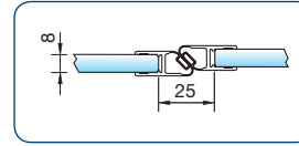
art. no. 8852KU7-8-2010 sealing profile for glass-glass 180° for 6 and 8 mm glass for a shower hinge opening to one side
