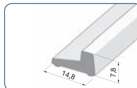
art. no. 8590E6EV5-2010 splash protection profile square cut length 2010 mm with sealing profile 8864KU0-8-2010
