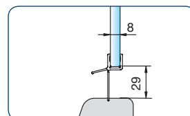
art. no. 8866KU0-8-2010 for 6 and 8 mm glass
