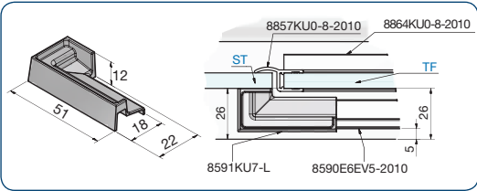
art. no. 8591KU7-L cover cap left
