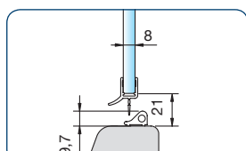
art. no. 8868KU0-8-R500 for 6 and 8 mm glass in combina- tion with curved splash guard for tub radius R500-550 winding off = 1194 mm (art. no. 8881 and 8882-R500)
