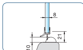
art. no. 8864KU0-8-2010 for 6 and 8 mm glass in combina- tion with acrylic semi-circular rod (art. no. 8539KU5, radius = 10 mm)
