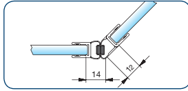
art. no. 8875KU7-8-2010 sealing profile for glass-glass 135° for 6 and 8 mm glass for an inward and outward opening shower hinge
